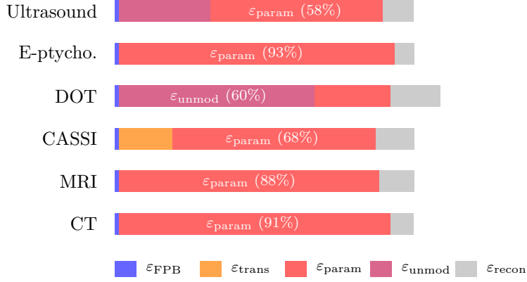
Figure 4. Error decomposition by modality. Stacked bars show the relative contribution of each Theorem 1 error term for 6 representative modalities. For well-conditioned systems (CT, MRI, e-ptychography), parameter mismatch \epsilon_{\text{param}} dominates and is reducible by calibration. For scattering-dominated systems (DOT), unmodeled physics \epsilon_{\text{unmod}} dominates and requires tier-lifting. \epsilon_{\text{FPB}} < 1\% in all cases. \epsilon_{\text{spec}} = \epsilon_{\text{trans}} = 0 for 31/36 modalities; CASSI shows nonzero \epsilon_{\text{trans}} due to dispersion-accumulation chain ambiguity.
