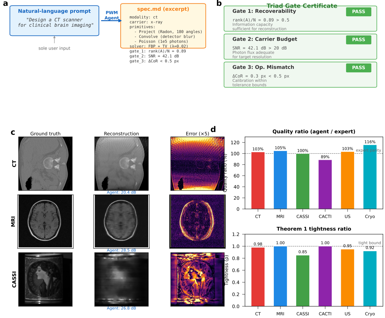
Figure 4: Design-to-real validation. a , A natural-language prompt (sole user input) and the agent-generated spec.md excerpt for CT. b , Triad gate certificate: all three diagnostic gates pass with quantitative margins. c , Ground truth, agent reconstruction, and amplified absolute difference ( 5\times , inferno colormap) for three real-data modalities spanning X-ray (CT), spin (MRI), and photon (CASSI) carriers. Both methods receive only measurements and calibration metadata. Agent/expert PSNR annotated below each reconstruction. d , Quality ratio relative to expert base-lines (top; 100% = expert parity) and Theorem 1 tightness ratio (bottom; values near 1 indicate tight bounds) across all 6 real-data modalities.
