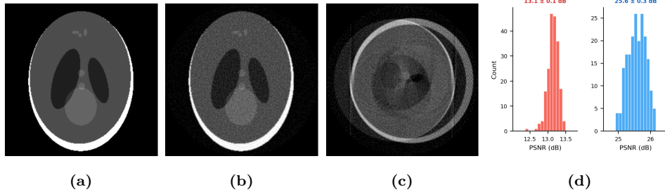
Figure 4. CT reconstruction comparison (modified Shepp–Logan phantom [32], 128 projections, Poisson noise, n = 200 ). (a) Ground truth. (b) Framework with Judge ( \in \mathfrak{S} verified): correct angular model, Ram-Lak filter, non-negativity enforced. (c) Without Judge: wrong angular range ( 360^\circ assumed instead of 180^\circ ), producing doubled edges and streak artifacts; 5,326 non-negativity violations. (d) PSNR distribution: with Judge 25.6 \pm 0.3 dB vs. without Judge 13.1 \pm 0.1 dB ( n = 200 , p < 10^{-30} , Wilcoxon).
