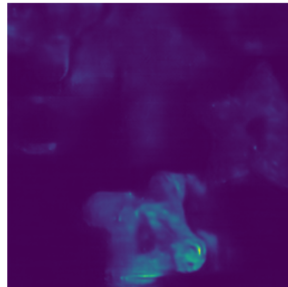
MST-L
