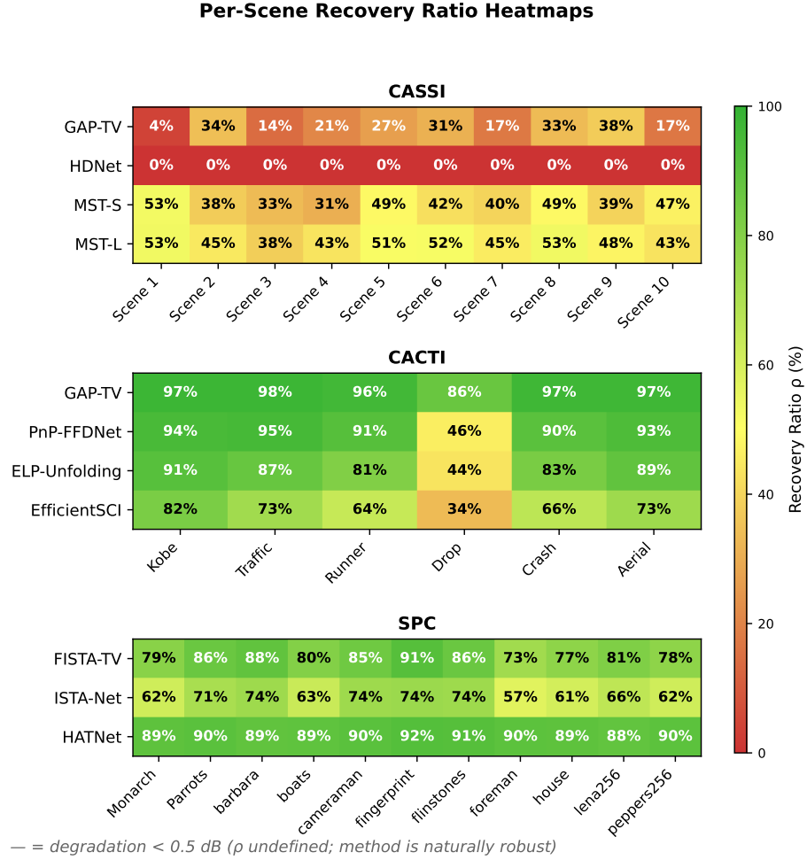
Fig. 2: Per-scene/video recovery ratio ( \rho ) heatmaps for CASSI (top, 10 scenes \times 4 methods), CACTI (middle, 6 videos \times 4 methods), and SPC (bottom, 11 images \times 3 methods). Red indicates low recovery; green indicates high recovery. Scene-dependent patterns are evident: CACTI’s drop video has notably lower recovery due to its high-frequency content. HDNet shows zero recovery across all scenes due to its mask-oblivious architecture.
