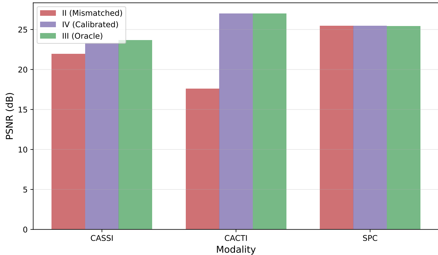
Scenario IV: Grid-Search Calibration vs Oracle
