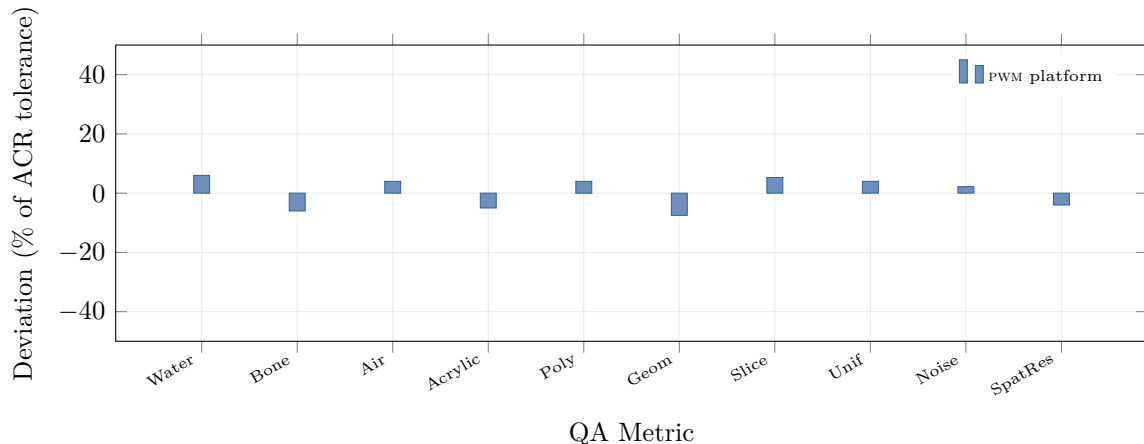
Figure 4: Metric deviations from nominal values on an ACR CT 464 phantom scan (GE Revolution Apex, 120 kVp, 5 mm axial), expressed as percentage of the respective ACR tolerance for each metric. All continuous metrics fall within \pm 8\% of their tolerances, well below the \pm 100\% action boundary. Low-contrast detectability (5/5 targets) and artifact evaluation (score 0) are discrete metrics shown in Table 2.
