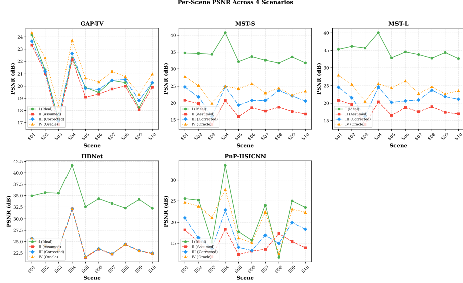
Fig. 3: Per-scene PSNR across four scenarios for each method. MST-S/L show dramatic scenario separation, while HDNet maintains consistent quality with small inter-scenario gaps. Scene-to-scene variation reflects content-dependent difficulty.
