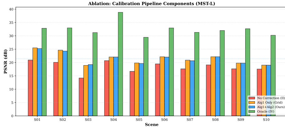
Fig. 5: Ablation study on MST-L: per-scene PSNR for No Correction (II), Grid-only (Alg1), Full pipeline (Alg1+Alg2), and Oracle (IV). Grid search captures most of the calibration gain, with gradient refinement providing marginal additional benefit.
