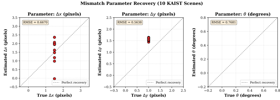
Fig. 2: Per-scene estimated vs. true mismatch parameters across 10 KAIST scenes. Dashed lines indicate ground truth values ( \Delta x=1.5 , \Delta y=1.0 , \theta=0.3^\circ ). The dispersion slope a_1 is recovered most accurately (RMSE=0.134 px/band).
