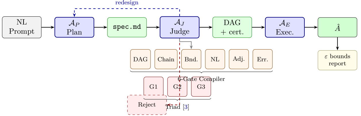
Figure 3. Specification-driven design pipeline. A natural-language prompt is the sole user input. \mathcal{A}_P generates a spec.md ; \mathcal{A}_J validates in two stages: a 6-gate compiler ( \text{DAG} \rightarrow \varepsilon_{\text{spec}} , \text{Chain} \rightarrow \varepsilon_{\text{trans}} , \text{Bounds} \rightarrow \text{complexity} , \text{NL} \rightarrow \varepsilon_{\text{param}} , \text{Adj.} \rightarrow \text{consistency} , \text{Err.} \rightarrow \varepsilon_{\text{FPB}} ) plus 3 Triad gates [3] (G1: recoverability, G2: carrier budget, G3: operator mismatch); rejected designs trigger redesign (dashed blue, up to 3 rounds). \mathcal{A}_E executes reconstruction and outputs \hat{A} with an explicit \varepsilon -bound report. See Figure 4 for per-modality error breakdown.
