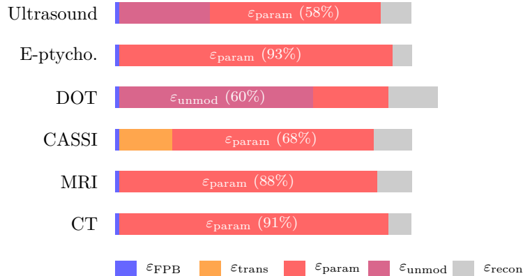
Figure 4. Error decomposition by modality. Stacked bars show the relative contribution of each Theorem 1 error term for 6 representative modalities. For well-conditioned systems (CT, MRI, e-ptychography), parameter mismatch \epsilon_{\text{param}} dominates and is reducible by calibration. For scattering-dominated systems (DOT), unmodeled physics \epsilon_{\text{unmod}} dominates and requires tier-lifting. \epsilon_{\text{FPB}} < 1\% in all cases. \epsilon_{\text{spec}} = \epsilon_{\text{trans}} = 0 for 31/36 modalities; CASSI shows nonzero \epsilon_{\text{trans}} due to dispersion-accumulation chain ambiguity.
