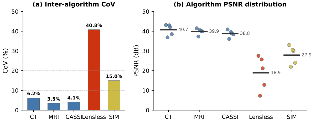
Figure 5. Specification dominance across 5 established modalities. (a) Inter-algorithm PSNR Coefficient of Variation (CoV) for the top-5 published reconstruction algorithms per modality. Well-conditioned systems (blue, \text{CoV} \approx 3.5\text{--}6.2\% ) show that the top algorithms converge tightly—the forward-model specification constrains the quality ceiling. SIM shows moderate CoV (15.0%). Ill-conditioned compressive systems (red, \text{CoV} > 40\% ) require careful algorithm selection. (b) Individual algorithm PSNR values (dots) with mean (horizontal bar) for each modality. Tight clusters for CT/MRI/CASSI confirm specification dominance; wide spread for Lensless shows algorithm sensitivity. Data from Extended Data Table 7.
