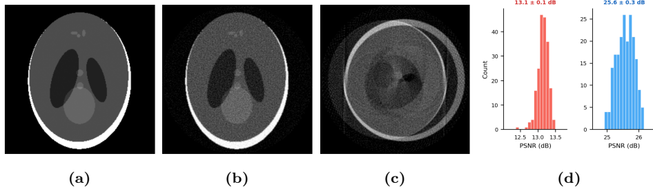
Figure 4. CT reconstruction comparison (modified Shepp–Logan phantom [32], 128 projections, Poisson noise, n = 200 ). (a) Ground truth. (b) Framework with Judge ( \in \mathfrak{S} verified): correct angular model, Ram-Lak filter, non-negativity enforced. (c) Without Judge: wrong angular range ( 360^\circ assumed instead of 180^\circ ), producing doubled edges and streak artifacts; 5,326 non-negativity violations. (d) PSNR distribution: with Judge 25.6 \pm 0.3 dB vs. without Judge 13.1 \pm 0.1 dB ( n = 200 , p < 10^{-30} , Wilcoxon).
