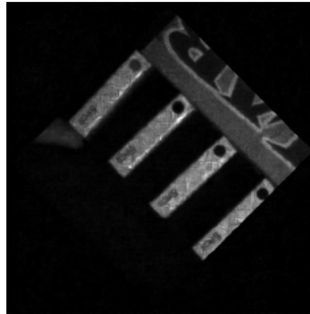
EfficientSCI (calibrated)
