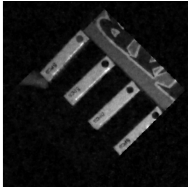
GAP-TV (calibrated)
