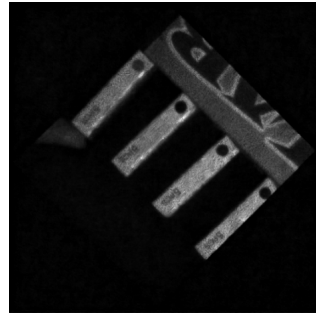
EfficientSCI (mismatched)
