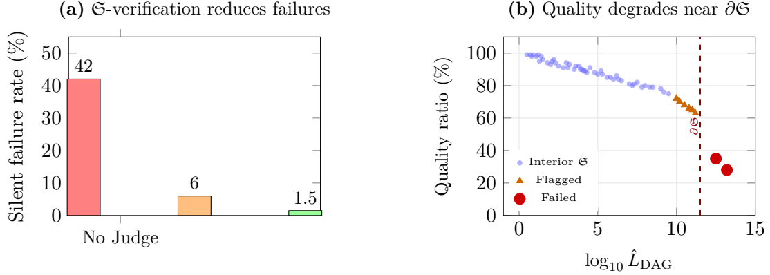
Figure 5. Failure analysis across 134 test cases. (a) \mathfrak{S} -verification reduces silent failures in two stages: pre-execution gates (42% \rightarrow 6%) and post-execution quality audit (6% \rightarrow 1.5%). (b) Quality ratio vs. estimated Lipschitz constant \hat{L}_{\text{DAG}} (log scale). The two residual failures (red) occur at \partial\mathfrak{S} —bifurcation points where \hat{L}_{\text{DAG}} \rightarrow \infty —while all interior- \mathfrak{S} problems (blue) achieve \geq 75\% quality. Orange triangles: flagged by quality audit. The dashed line indicates the empirical boundary where certifiability (S4) degrades.
