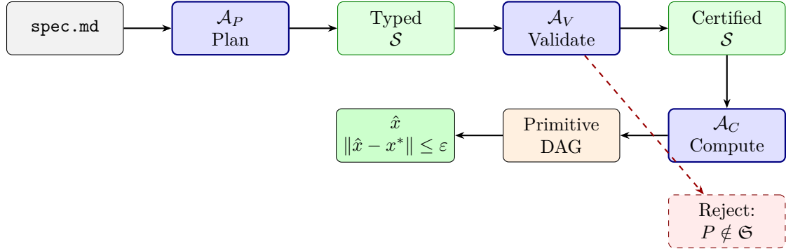
Figure 2. Specification-centered pipeline. A spec.md is the sole input. \mathcal{A}_P (Plan) parses it into a typed specification and selects primitives. \mathcal{A}_V (Validation) checks well-posedness and classifies the problem within \mathfrak{S} or rejects it. \mathcal{A}_C (Computation) constructs a primitive DAG and executes it.
