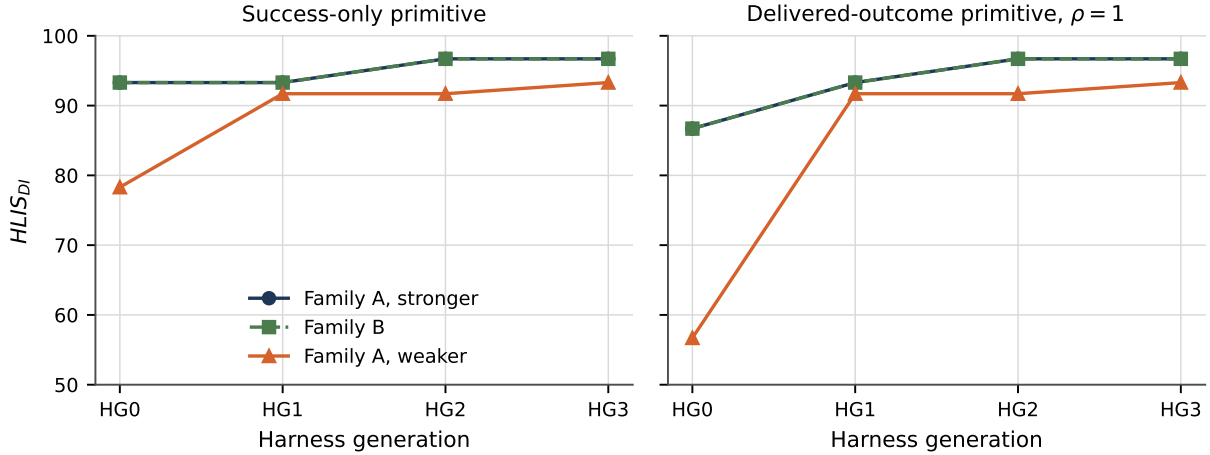
Figure 2: The three Harness Scaling Curves of Table 38 under the success-only primitive (left) and the delivered-outcome primitive at \rho = 1 (right). Families A (stronger) and B coincide on both panels. The HG0→HG1 step is invisible on the left and is the largest movement on the right.
