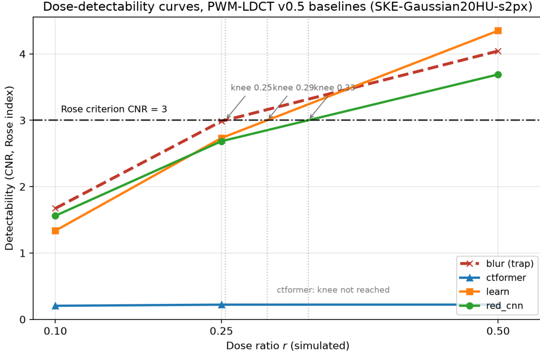
Figure 4: Dose-detectability curves. CNR (mean over a fixed multi-seed set, n = 30 test slices per dose level) versus simulated dose ratio for the four baselines and the standing Gaussian-blur trap, with the Rose criterion (CNR = 3.0) drawn as the reference line. The knee (the dose at which the interpolated CNR crosses the Rose criterion) is reached by RED-CNN at dose ratio \approx 0.33 , by LEARN at \approx 0.29 , and by the blur trap at \approx 0.25 ; CTformer stays below the Rose criterion at all three dose points (CNR \approx 0.52 – 1.44 after retraining), so its knee is not reached in the measured range. Single-point detectability claims are thus replaced by a curve statement: the dose at which each method becomes reliably detectable differs across baselines and is exactly the quantity the dataset is designed to expose (companion charter, Rung 4). The curves were produced by baselines/src/pwm_ldct_baselines/dose_curve.py from the committed per-model result JSONs and the corresponding statistics are released in output/dose_detectability_stats.json .
