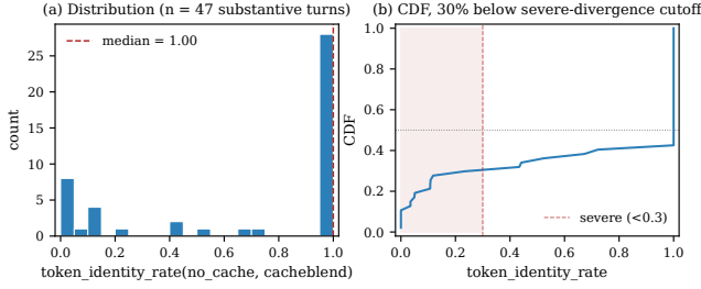
Figure 4: Distribution of token_identity_rate(no_cache, cacheblend) across 47 substantive ( \geq 256 -token prompt) turns at T = 0 . (a) Histogram: a mass at 1.0 (bit-identical) and a tail at 0–0.1 (severe divergence). (b) CDF: 30% of turns fall below the severe-divergence cutoff at 0.3. The middle bins are empirically rare; the distribution is sharply bimodal.
