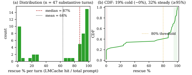
Figure 3: Per-turn rescue rate across the 47 substantive turns. (a) Histogram with median and mean overlaid: the bimodality is sharp — a mass near 0% (cold-cache first-turns of each capture plus pattern-shift turns where cacheblend’s LOOKUP cannot find a match) and a steady-state peak above 90%. (b) CDF: 19% of turns rescue near 0%, 32% reach \geq 95\% , the rest are distributed across the intermediate band.
