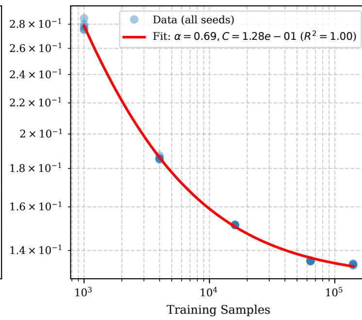
G1
