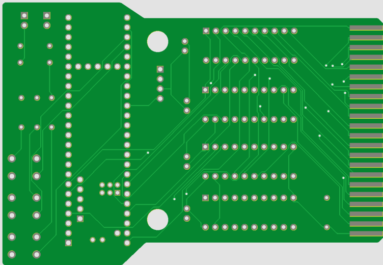
E1819670 PCB view BOTTOM (bottomview)
