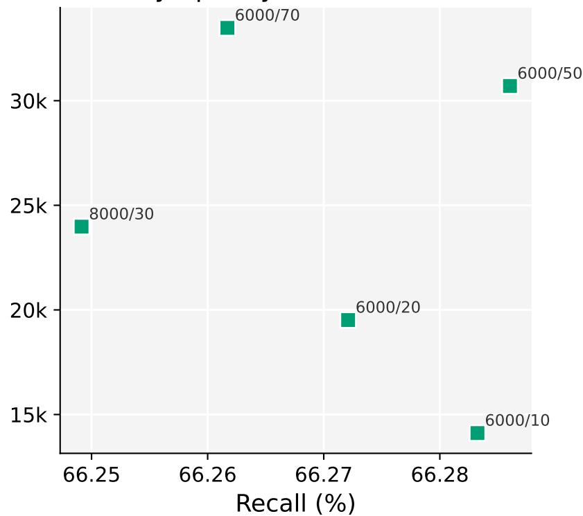
SymphonyQG-BriskSeed
