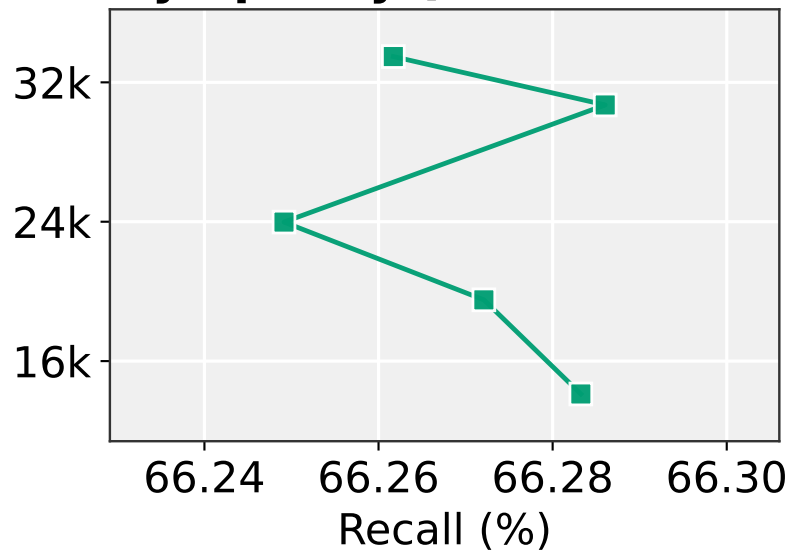
SymphonyQG-BriskSeed
