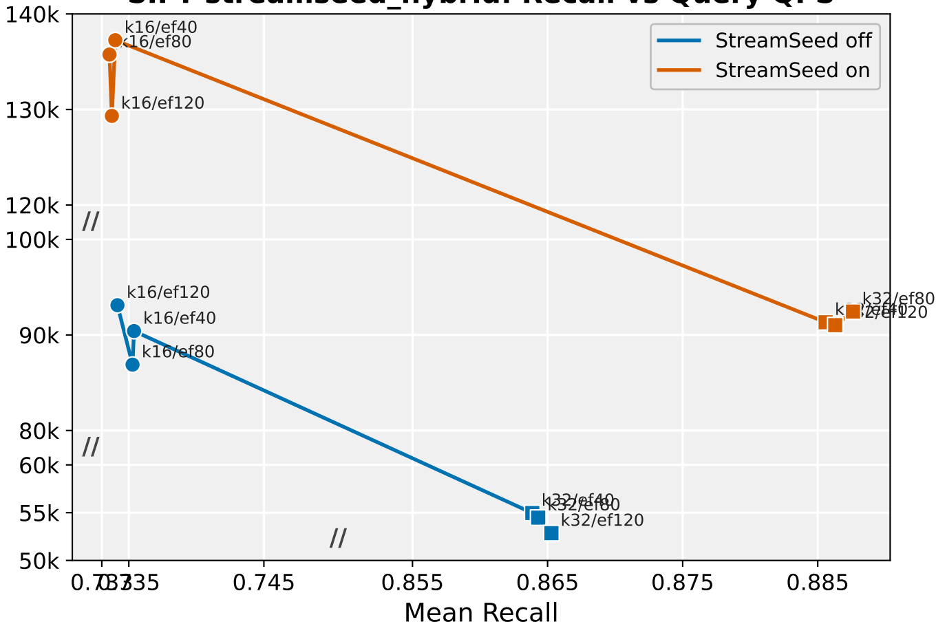
SIFT streamseed_hybrid: Recall vs Query QPS
