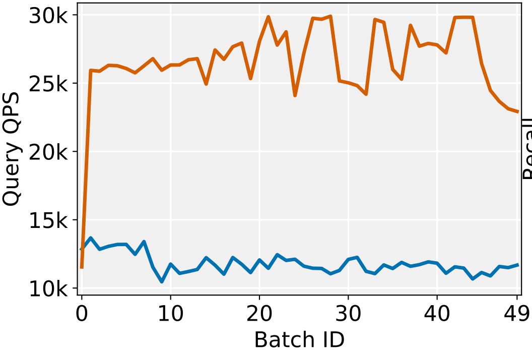
Query QPS
