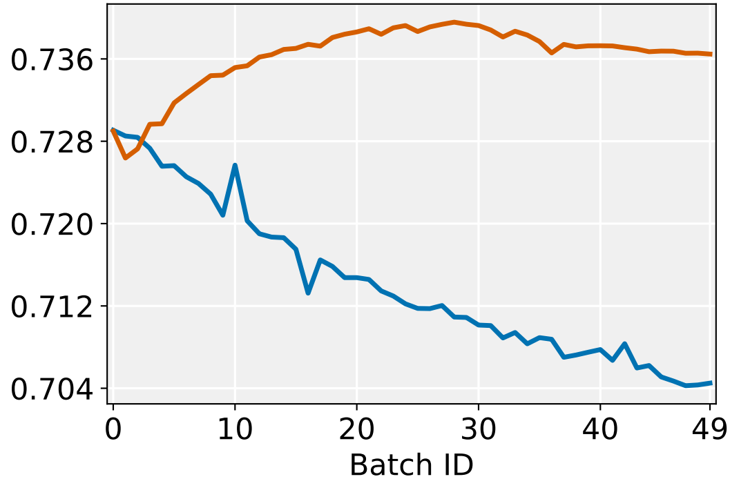
Recall
