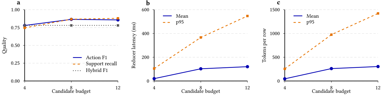
Figure 3. Measured action-reducer operating points over the frozen five-sample, nine-family matrix (135 rows per budget). (a) F1 and support-evidence recall; the dotted line is the 0.7801 hybrid F1. (b) all-row mean and p95 reducer latency. (c) all-row mean and p95 tokens, using provider usage when present and the recorded estimate otherwise. Four candidates truncate relations; eight maximize F1; twelve cost more without improving F1. Evidence: derived summaries of real-online rows.
