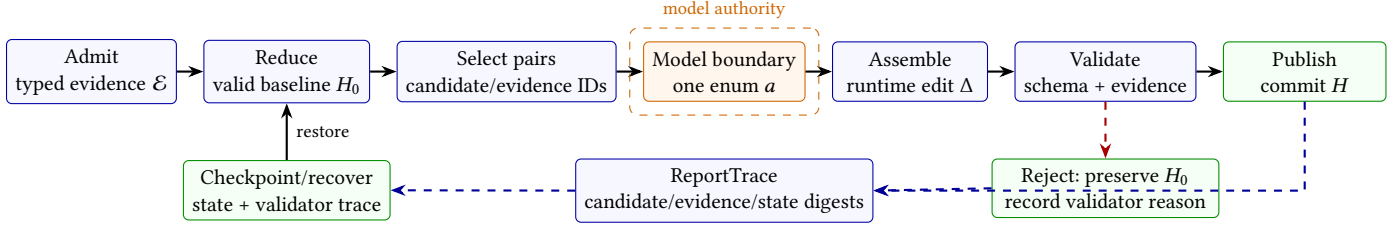
Figure 2. Concrete reducer invocation and recovery path. Only candidate descriptions and registered evidence IDs cross the model boundary, and the model returns one action enum. The runtime constructs \Delta , validates it, commits H or preserves H_0 , and records digests and validator outcomes for replay. Checkpoint recovery is exercised by the model-free contract path; real-online runs retain the compatible trace fields.
