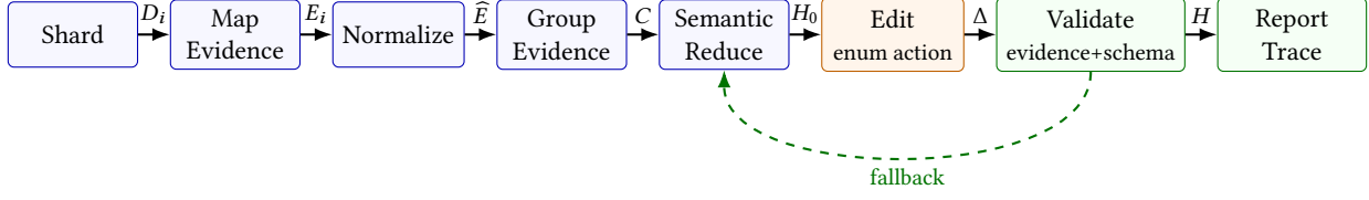
Figure 2. Operator-algebra view of Semantic MapReduce. The model-facing boundary is Edit, not full report generation: an LLM may choose a bounded action over candidates, while Validate remains system-owned and enforces evidence references, schema constraints, root/affected consistency, and fallback before ReportTrace.
