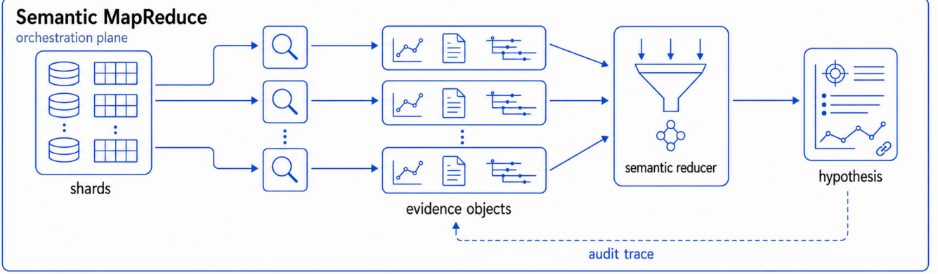
Figure 1. Motivating comparison. Naive stitching can connect telemetry, scripts, and an LLM agent, but it leaves the central systems question implicit: which shard-local symptoms should be merged into the same incident? Semantic MapReduce makes that boundary explicit. Shards produce evidence objects, a semantic reducer performs incident-level fusion, and the report carries audit links back to the evidence that supports each hypothesis.
