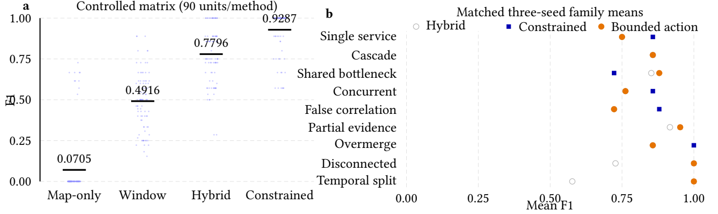
Figure 3. Working diagnostic, not a fair policy-selector result. (a) Individual F1 values and means for four incident/scenario-ID-blind policies over nine controlled families and ten seeds (90 units/method; simulation/model ); the constrained policy can read a generator-provided upstream hint. (b) Per-family means on 27 matched scenario-seed units: hybrid and legacy merge-only bounded-action values are real-online ; constrained values are simulation/model on identical generated evidence. The legacy action path edits semantic-graph H0, hybrid is a comparison/fallback policy, and constrained globally reclusters singleton evidence. The points therefore expose policy and permission differences; they are not task-matched SOTA peers. Figure evidence: derived-artifact .
