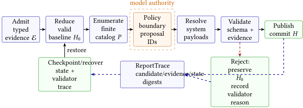
Figure 2. Concrete v2 reducer invocation and recovery path. The runtime constructs a finite catalog over registered candidates/evidence; a policy returns proposal IDs, never edit payloads. The runtime resolves and validates the selected batch, commits H atomically or preserves H_0 , and records catalog, selection, state, and validator digests. Checkpoint recovery is exercised by the model-free contract path. Historical real-online evidence predates this shared-catalog boundary and exercises merge/no-op v1 only.
