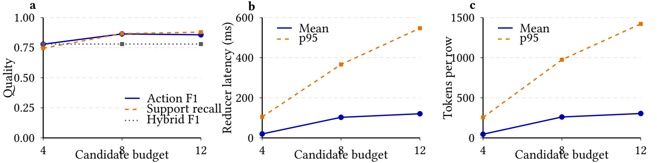
Figure 4. Measured action-reducer operating points over the frozen five-sample, nine-family matrix (135 rows per budget). (a) F1 and support-evidence recall; the dotted line is the 0.7801 hybrid F1. (b) all-row mean and p95 reducer latency. (c) all-row mean and p95 tokens, using provider usage when present and the recorded estimate otherwise. Four candidates truncate relations; eight maximize F1; twelve cost more without improving F1. Budget 8 was selected on this same historical matrix, so this is exploratory operating-point evidence rather than held-out tuning evidence. Evidence: derived summaries of real-online rows.
