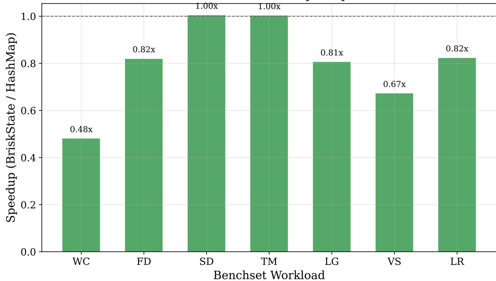
Benchset Relative Speedup
