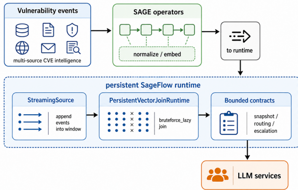
Figure 1: System overview of BRISKSNAPSHOT. A unified operator flow feeds vulnerability-intelligence events into a persistent SageFlow runtime, which maintains join-backed window state and exposes bounded contracts to downstream LLM-facing services.
