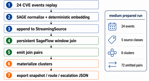
Figure 2: Live demonstration flow. The prepared replay drives one persistent SageFlow window-join runtime and exports snapshot, routing, and escalation contracts from the same maintained state.
