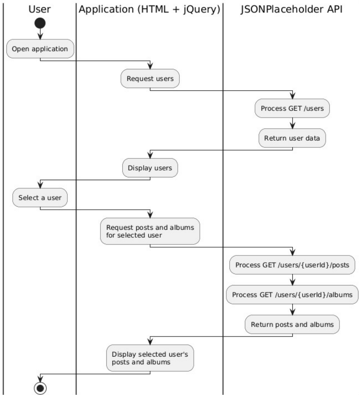
User Posts and Albums Viewer - Activity Diagram
