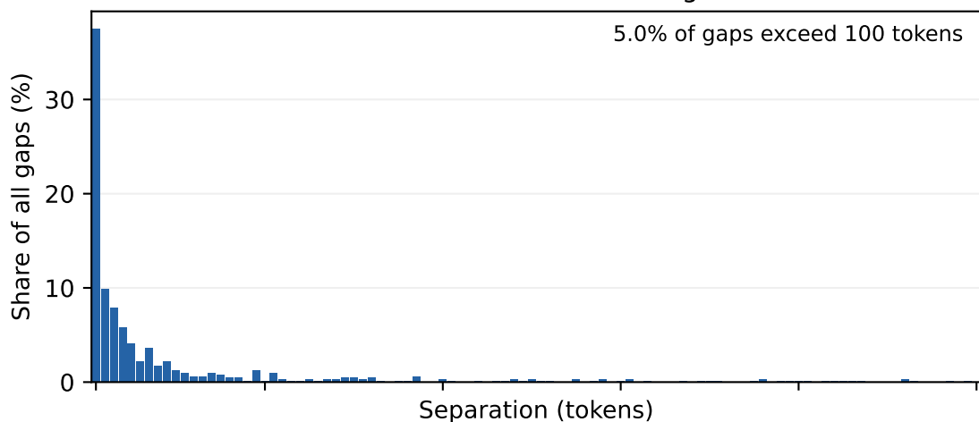
report — Distance between firing tokens
