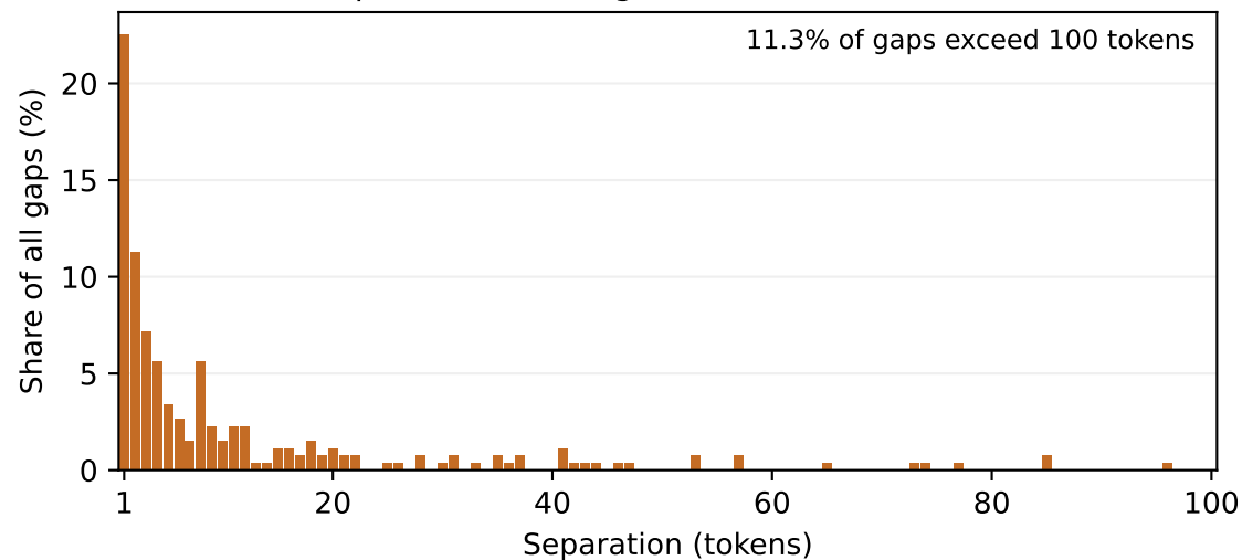
report — Non-firing tokens between bursts
