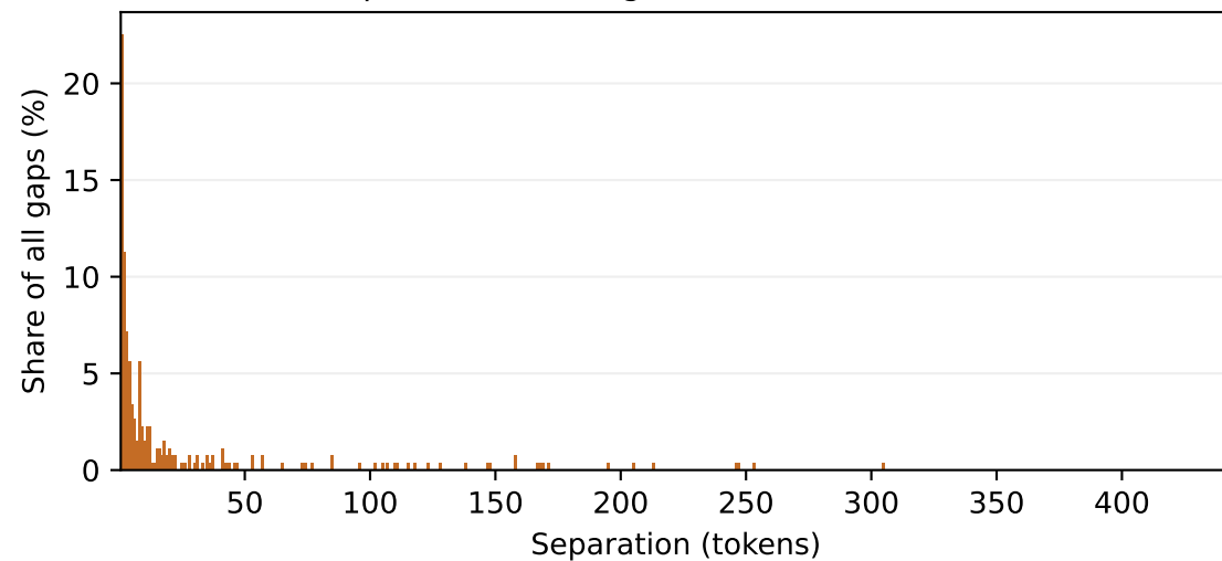
report — Non-firing tokens between bursts
