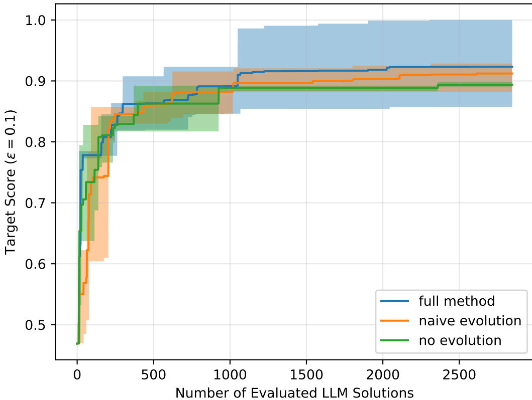
Component ablation for FirstAutocorrIneq
