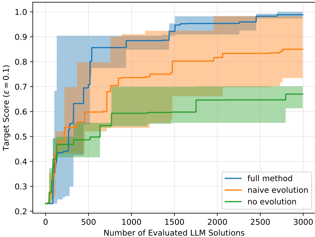
Component ablation for HexagonPacking( n=11 )
