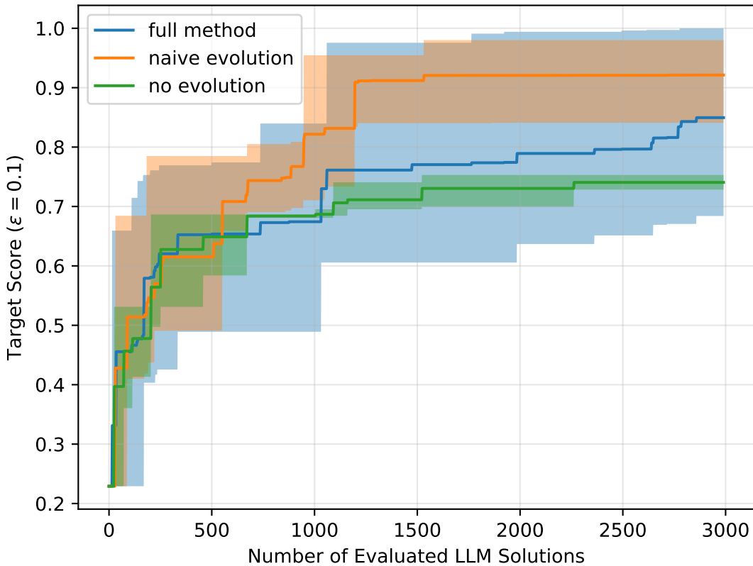
Component ablation for HexagonPacking( n=12 )
