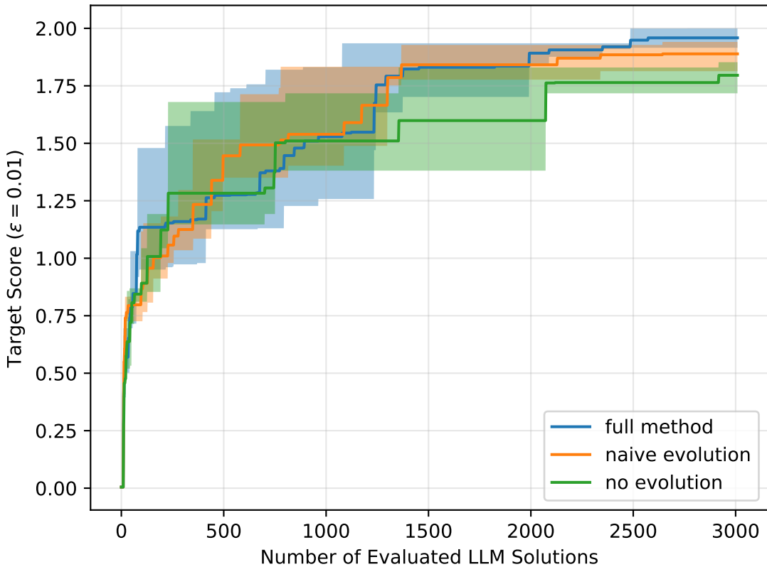
Component ablation for MinimizeMaxMinDist( n=16, d=2 )
