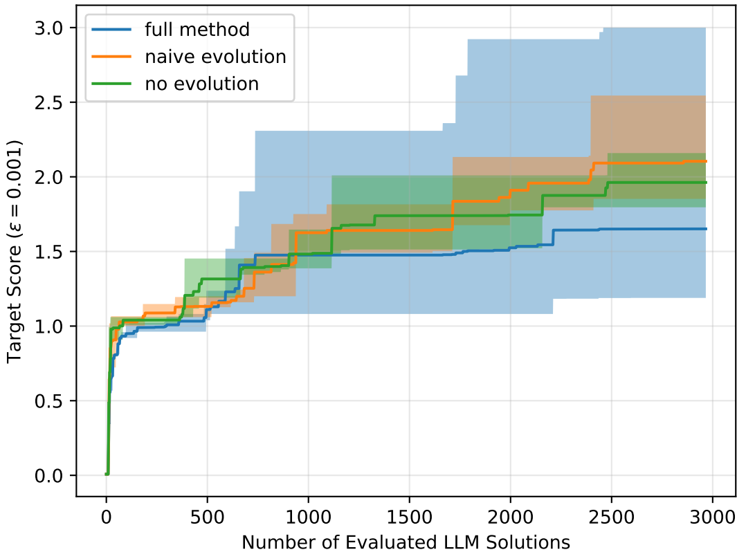
Component ablation for MinimizeMaxMinDist( n=14, d=3 )
