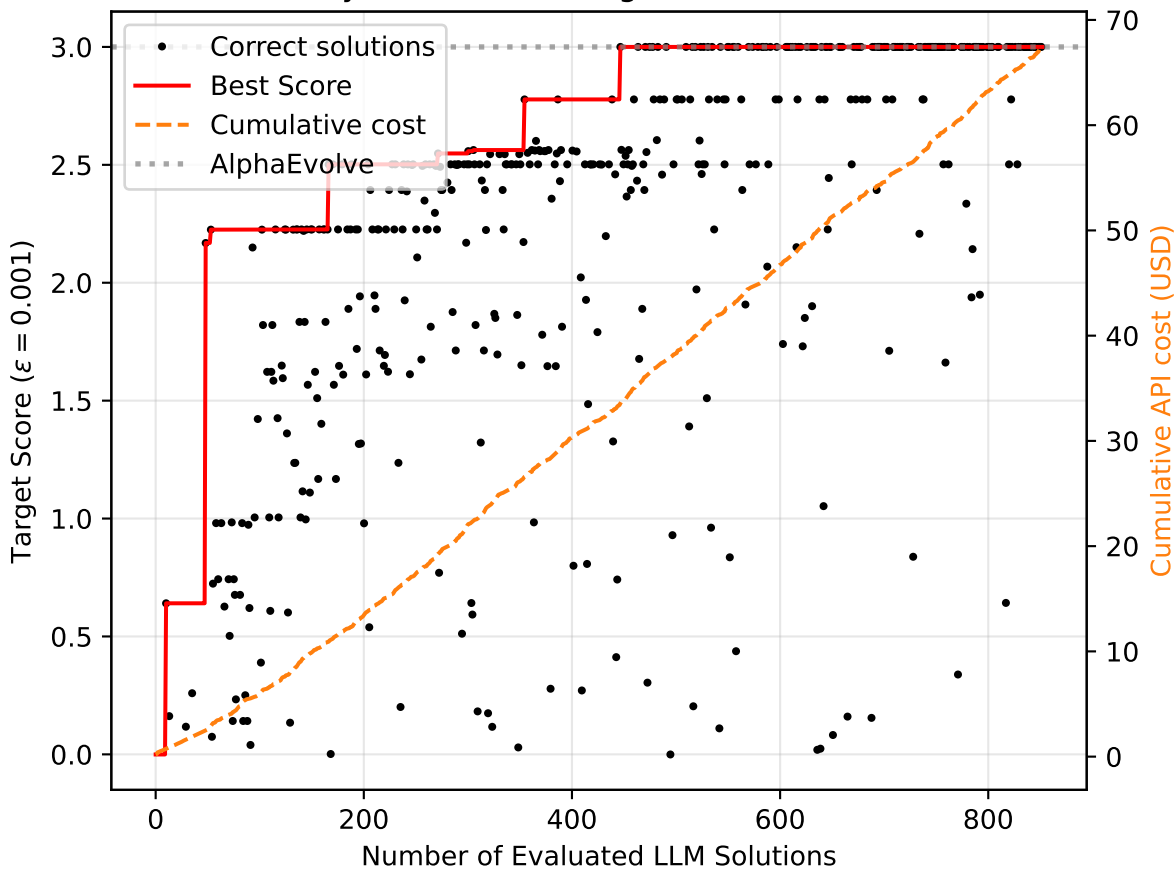
Solution history for CirclePackingRect(n=21) with GEMINI-2.5
