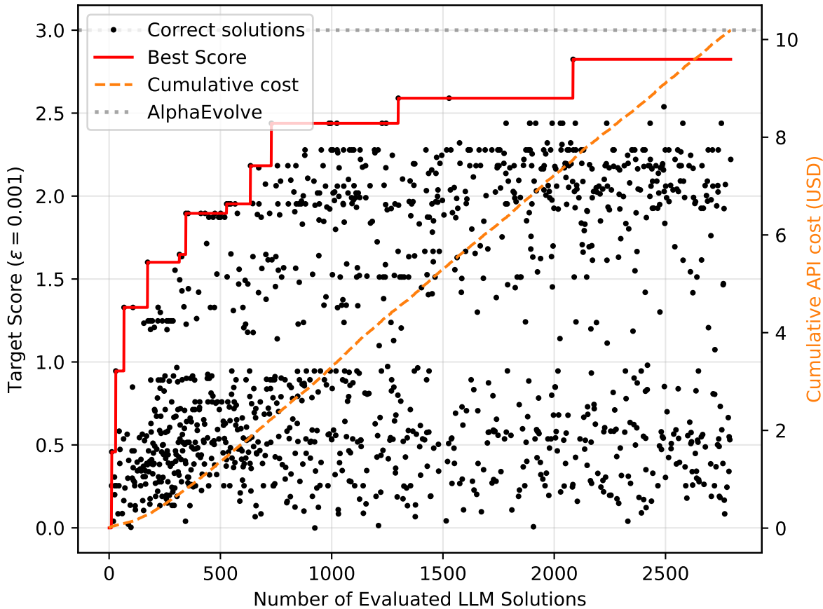
Solution history for CirclePackingRect(n=21) with Qwen3-Coder-30B
