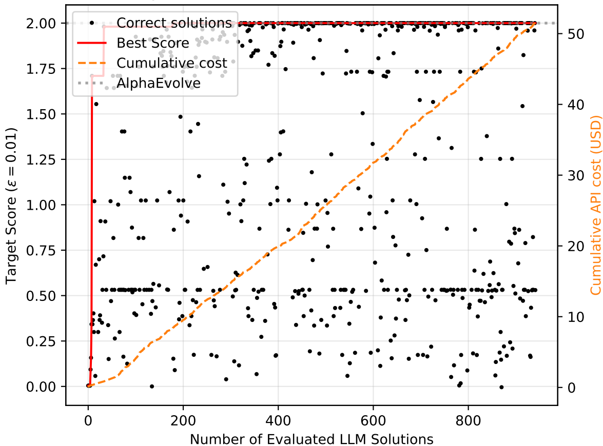
Solution history for MinimizeMaxMinDist( n=16, d=2 ) with GEMINI-2.5
