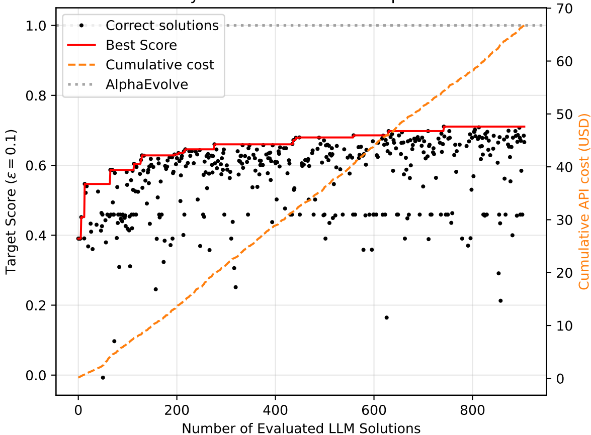
Solution history for SecondAutocorrIneq with GEMINI-2.5
