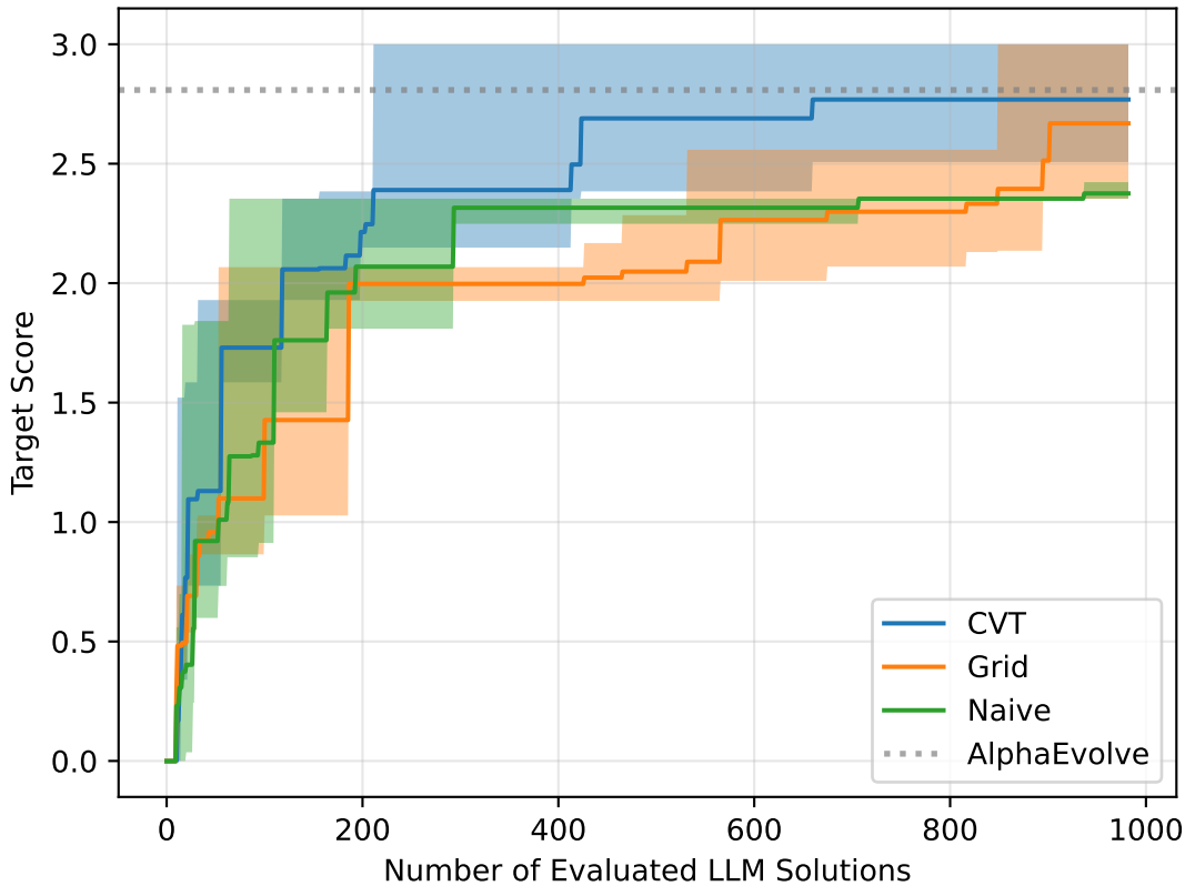
Elite selection ablation for CirclePackingSquare(n=32)
