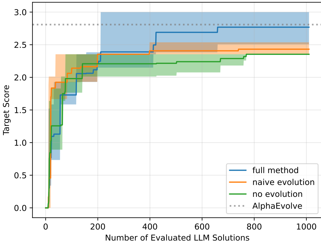
Component ablation for CirclePackingSquare(n=32)
