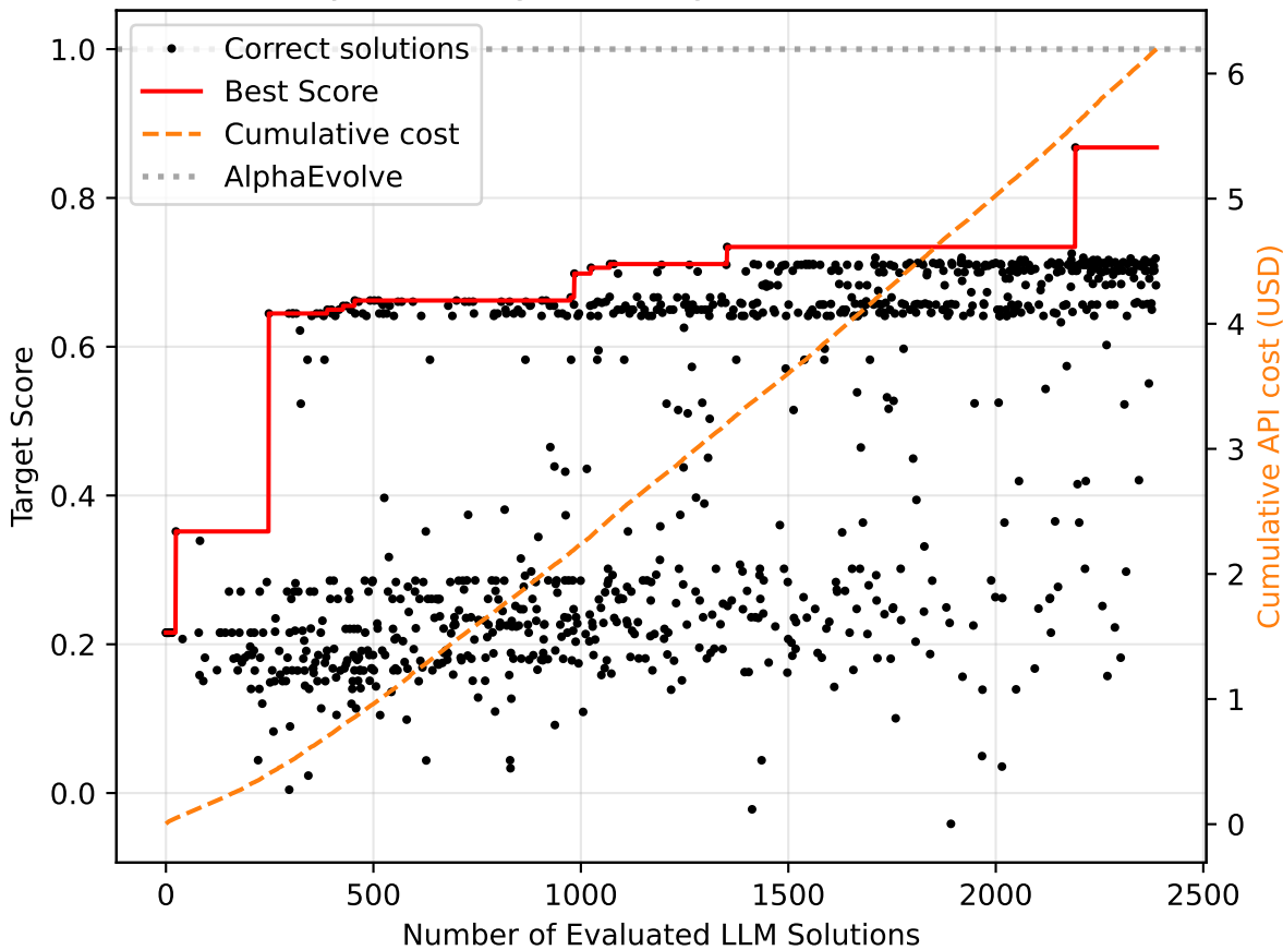
Solution history for HexagonPacking(n=11) with Qwen3-Coder-30B
