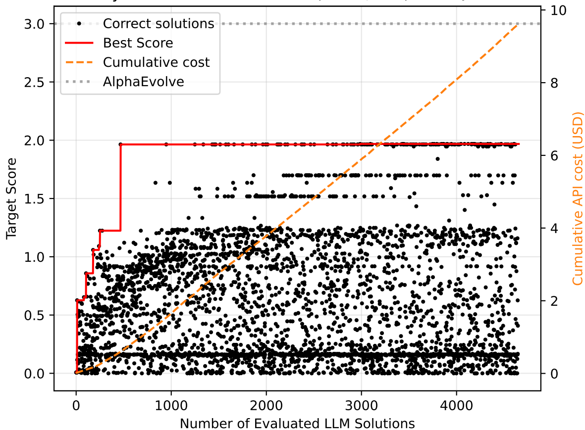
Solution history for MinimizeMaxMinDist( n=14, d=3 ) with Qwen3-Coder-30B
