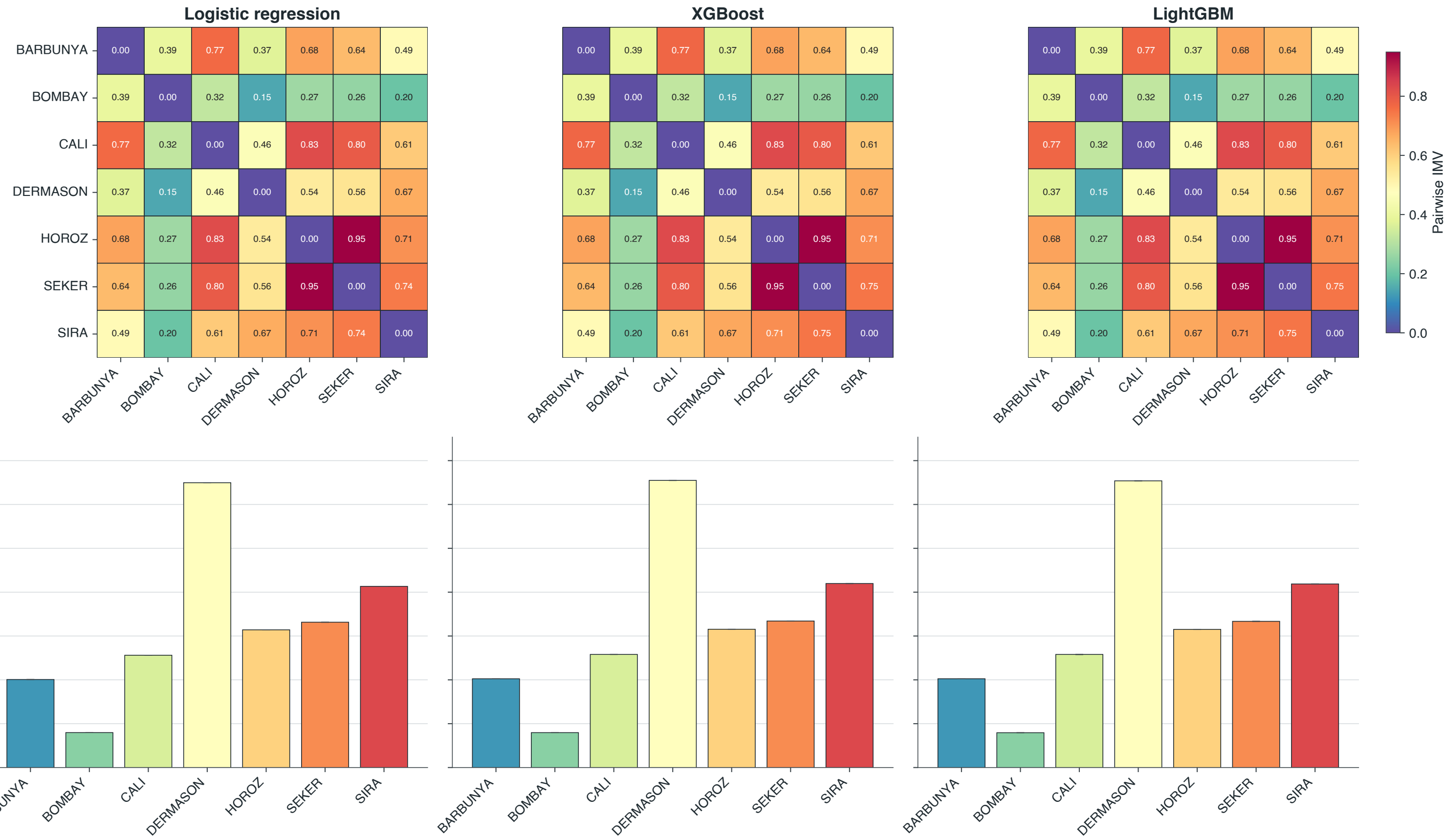
Dry Bean — pairwise IMV (top) and one-vs-rest IMV (bottom), mean over 10 seeds
