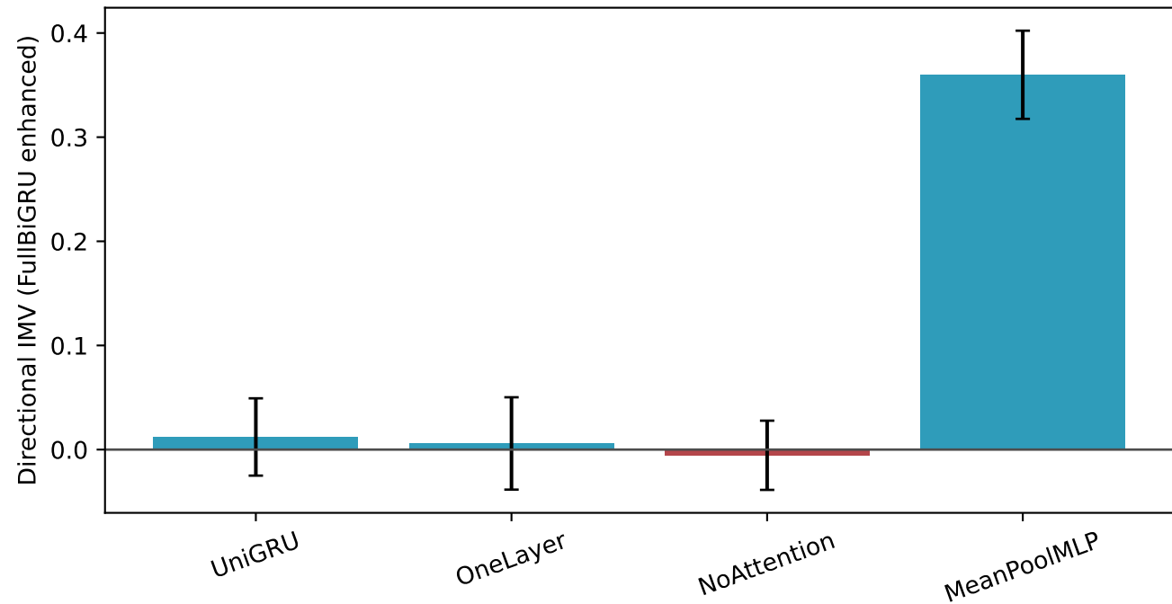
Full recurrent HAR model relative to each ablation
