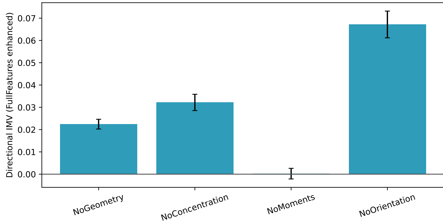
Full MAGIC Gamma model relative to each feature-group ablation
