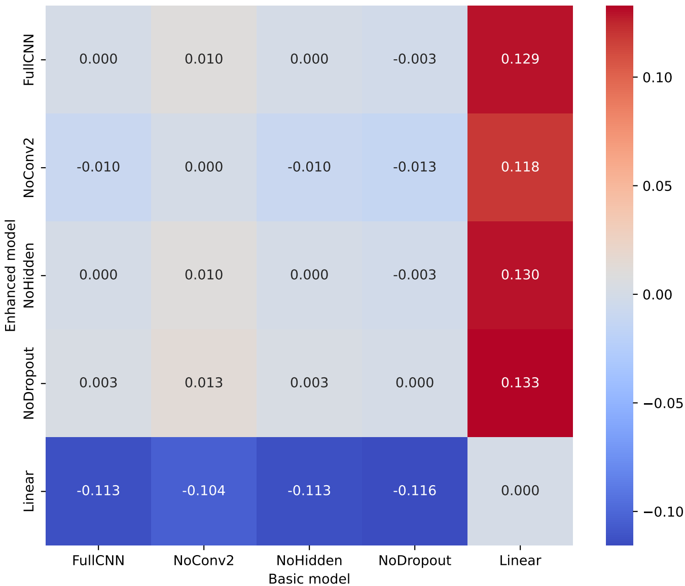
MNIST odd/even directional IMV, mean of 10 seeds
