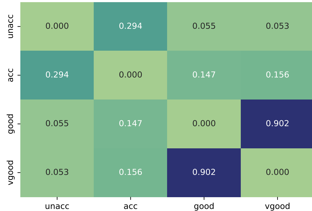
Car Evaluation (xgboost)
