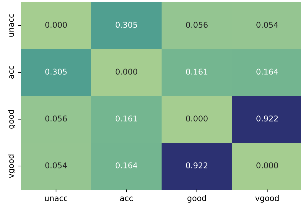
Car Evaluation (lightgbm)
