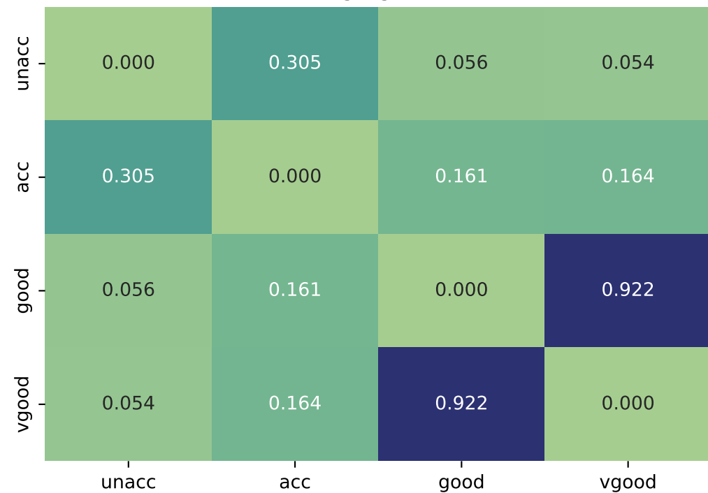
Car Evaluation (lightgbm)
